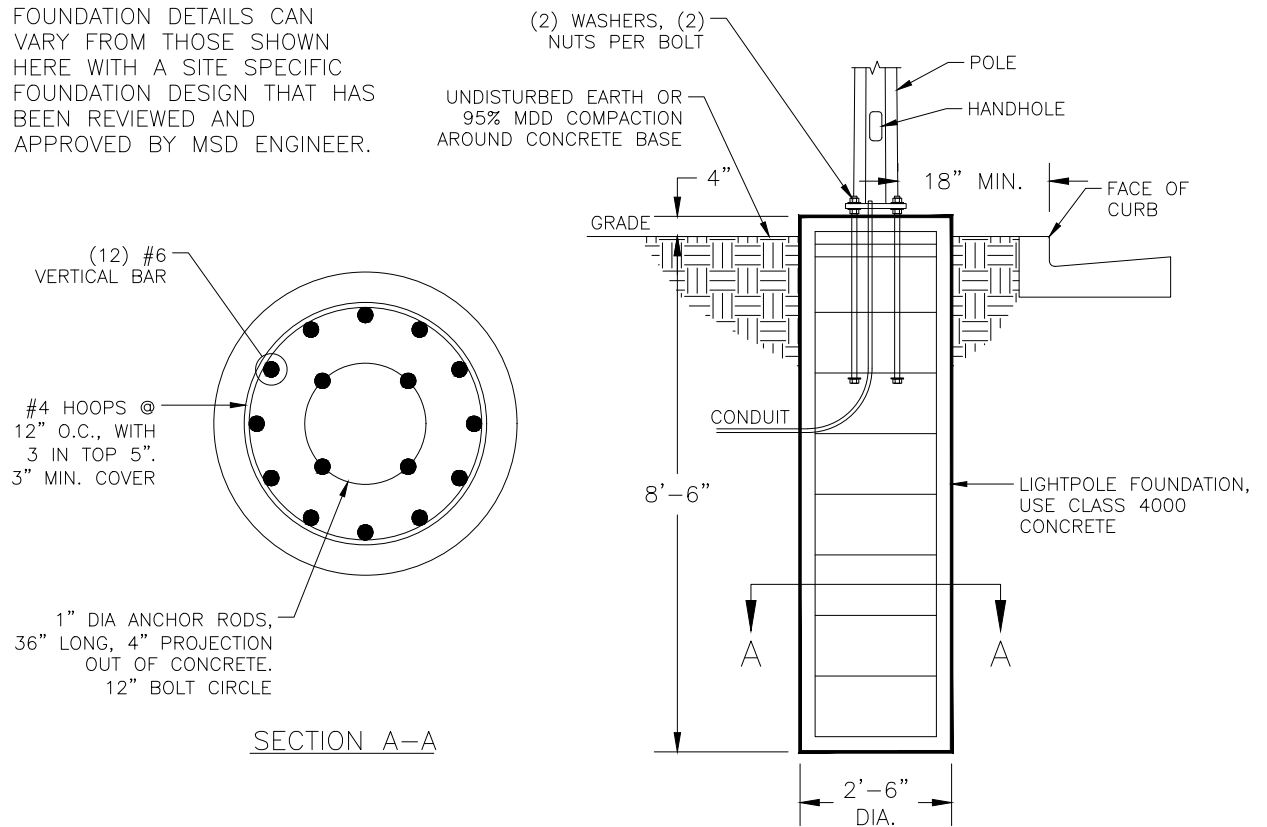
FOUNDATION DETAILS
